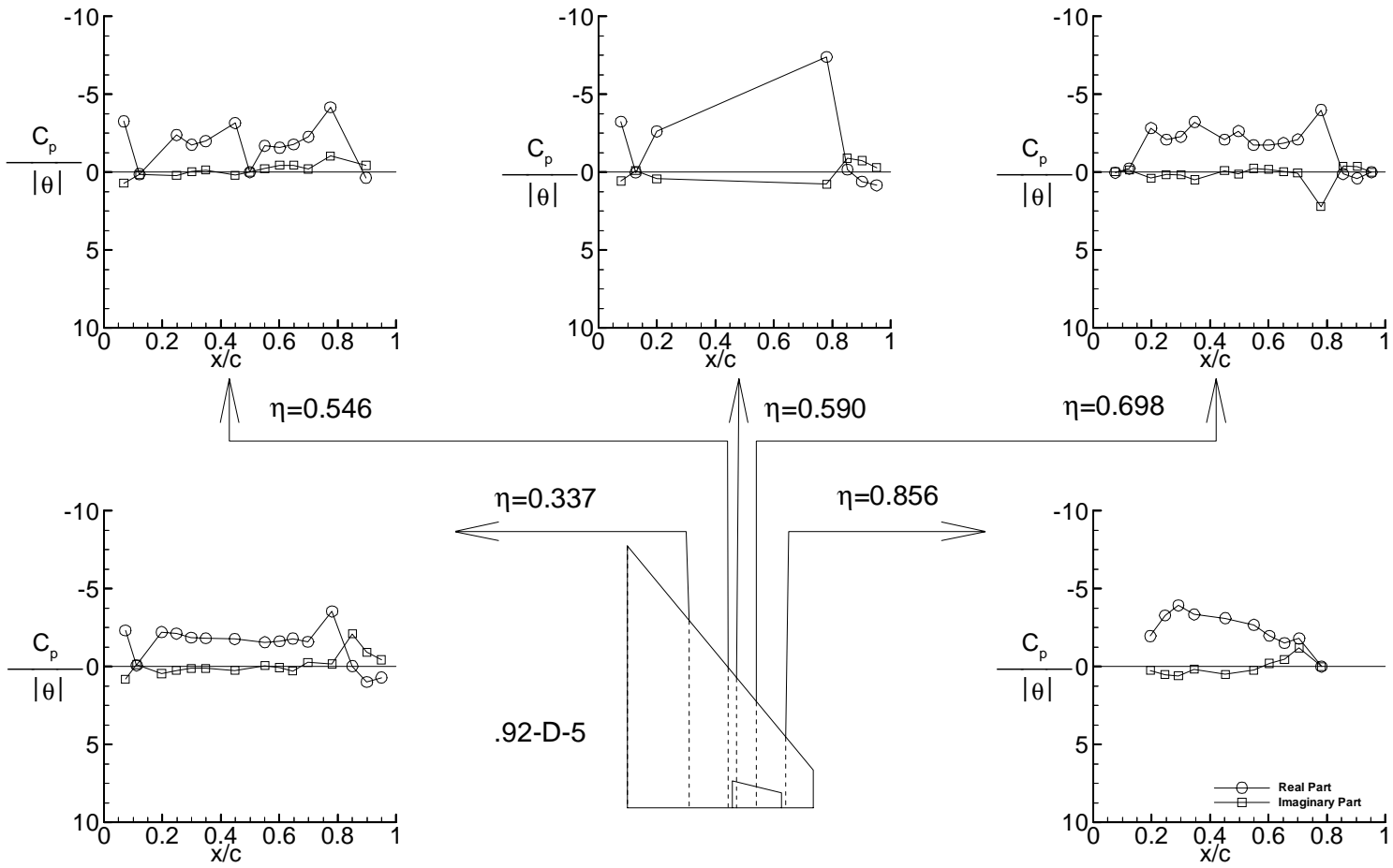
(d-2) Plot of data for test case 9E26 (point.92-D-5) Figure 6. Continued.
