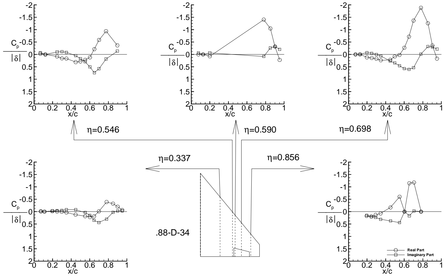
(n-2) Plot of data for test case 9E36 (point.88-D-34) Figure 6. Continued.
