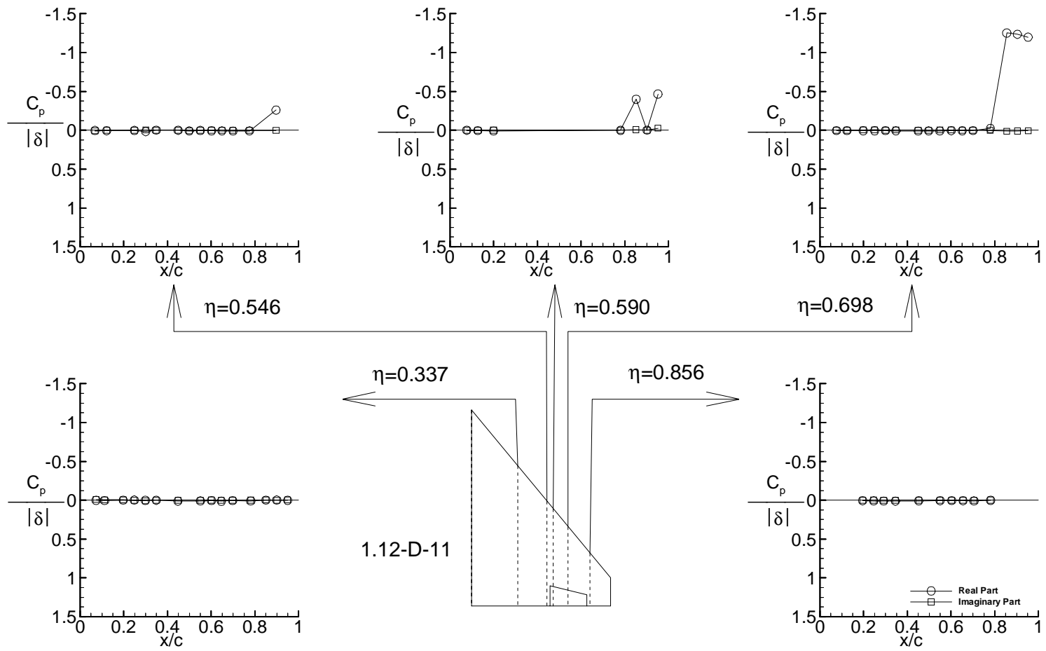
(s-2) Plot of data for test case 9E41 (point 1.12-D-11) Figure 6. Continued.
