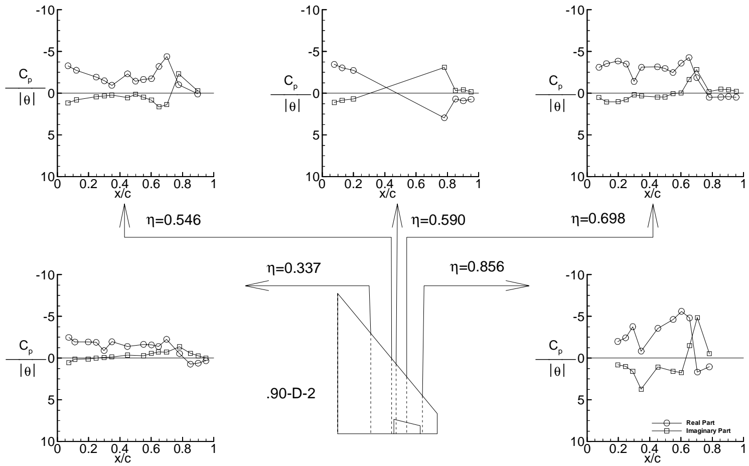
(h-2) Plot of data for test case 9E30 (point.90-D-2) Figure 6. Continued.
