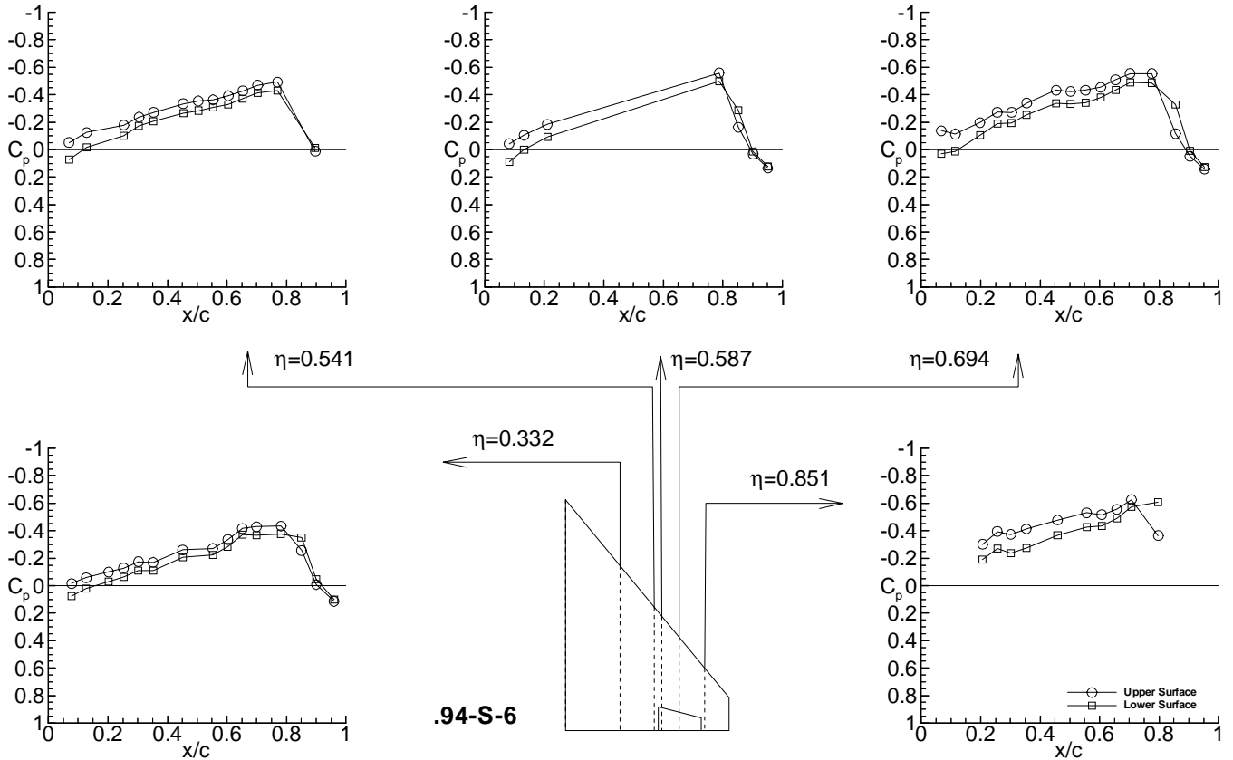
(j) Test case 9E10 (point .94-S-6) Figure 5. Continued.
