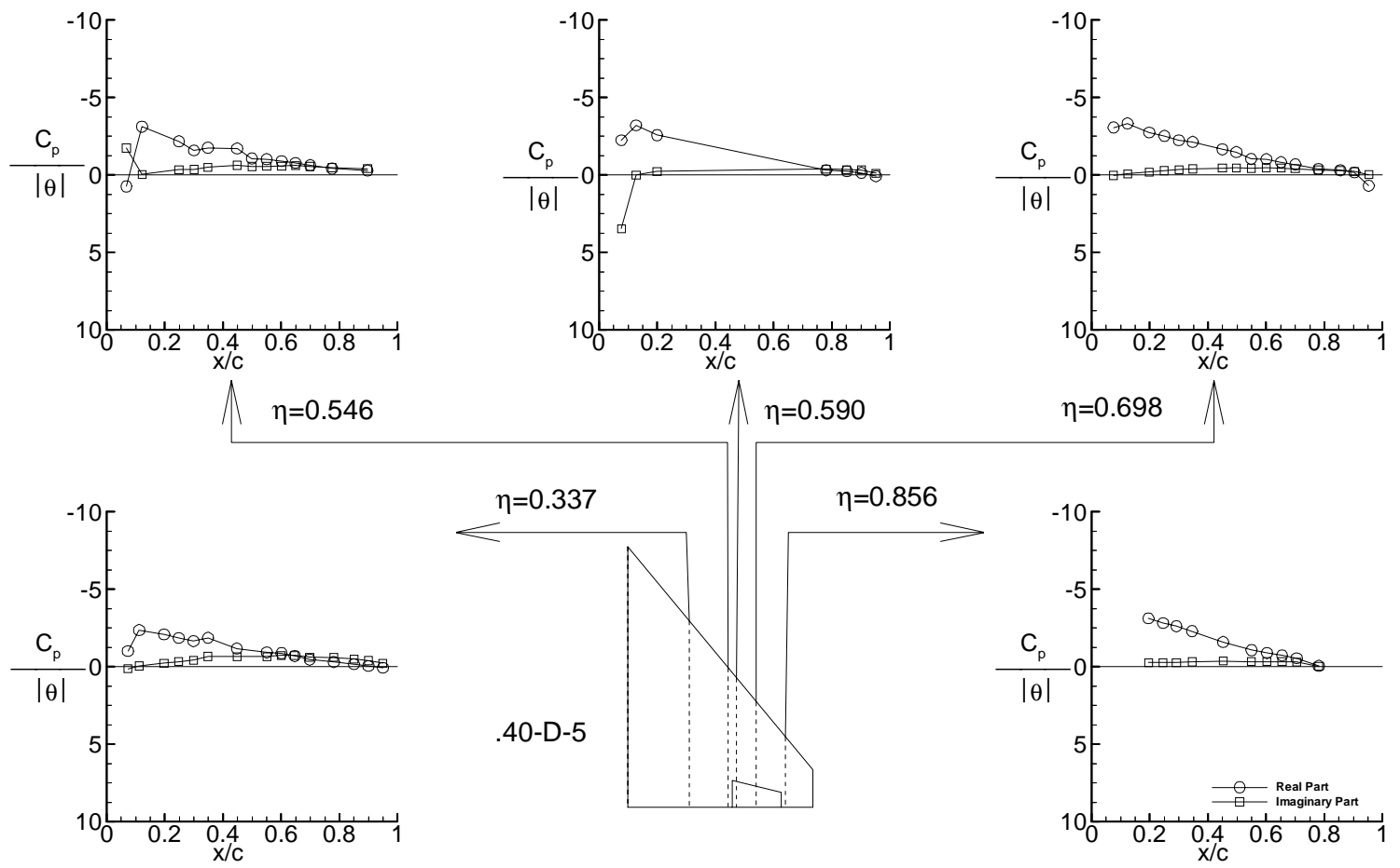
(a-2) Plot of data for test case 9E23 (point .40-D-5) Figure 6. Continued.
