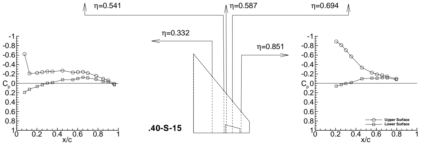
(m) Test case 9E13 (point .40-S-15) Figure 5. Continued.
