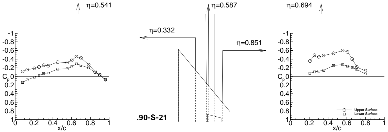
(u) Test case 9E21 (point .90-S-21) Figure 5. Continued.
