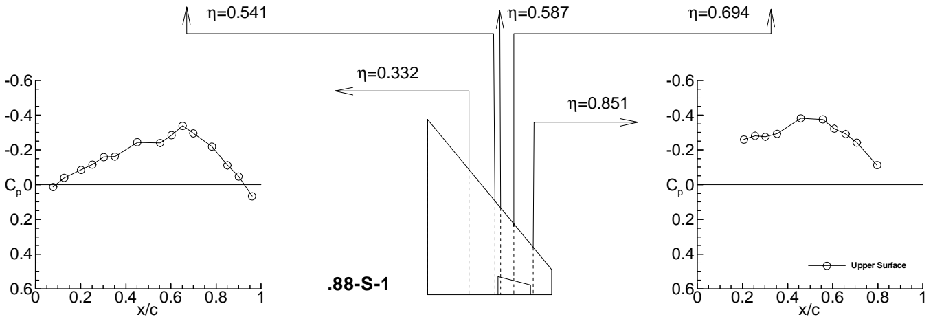
(b) Test case 9E2 (point .88-S-1) Figure 5. Continued.
