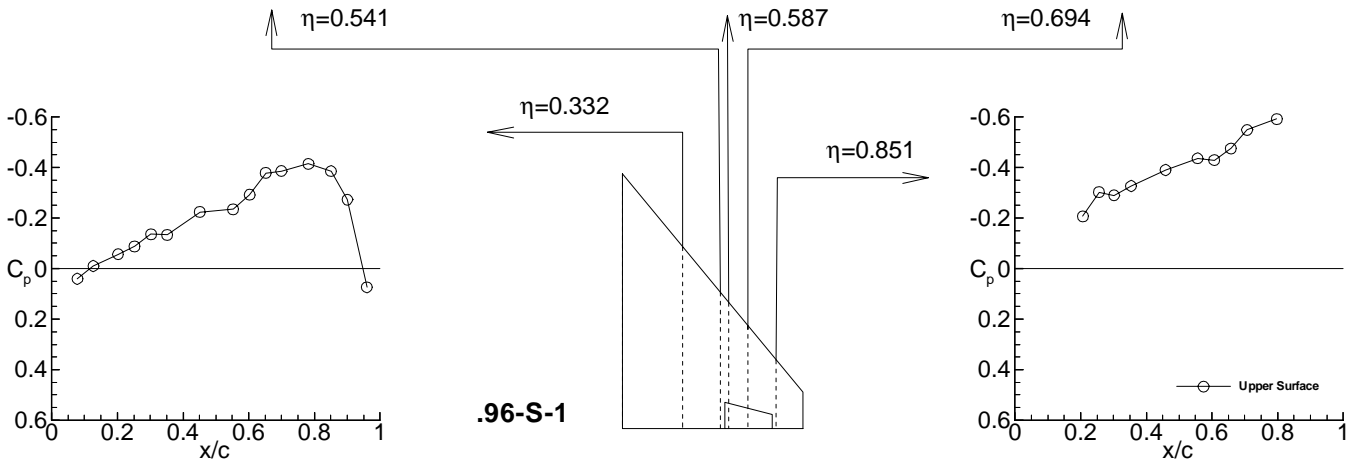
(f) Test case 9E6 (point .96-S-1) Figure 5. Continued.
