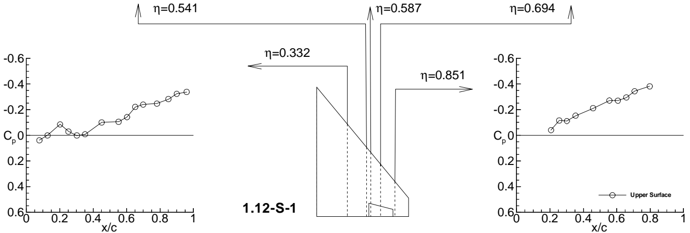
(g) Test case 9E7 (point 1.12-S-1) Figure 5. Continued.
