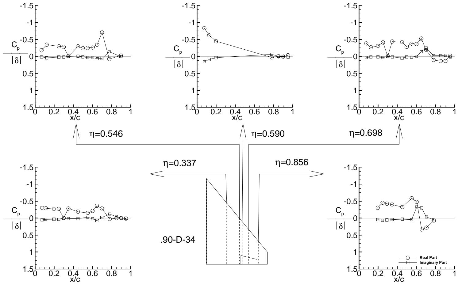
(v-2) Plot of data for test case 9E44 (point.90-D-34) Figure 6. Continued.
