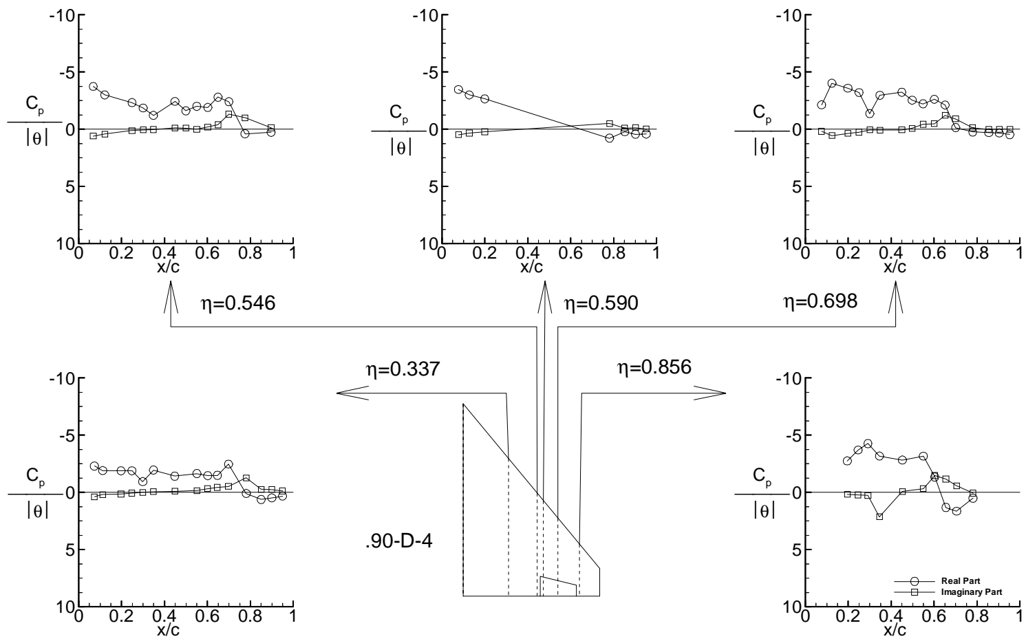
(i-2) Plot of data for test case 9E31 (point.90-D-4) Figure 6. Continued.
