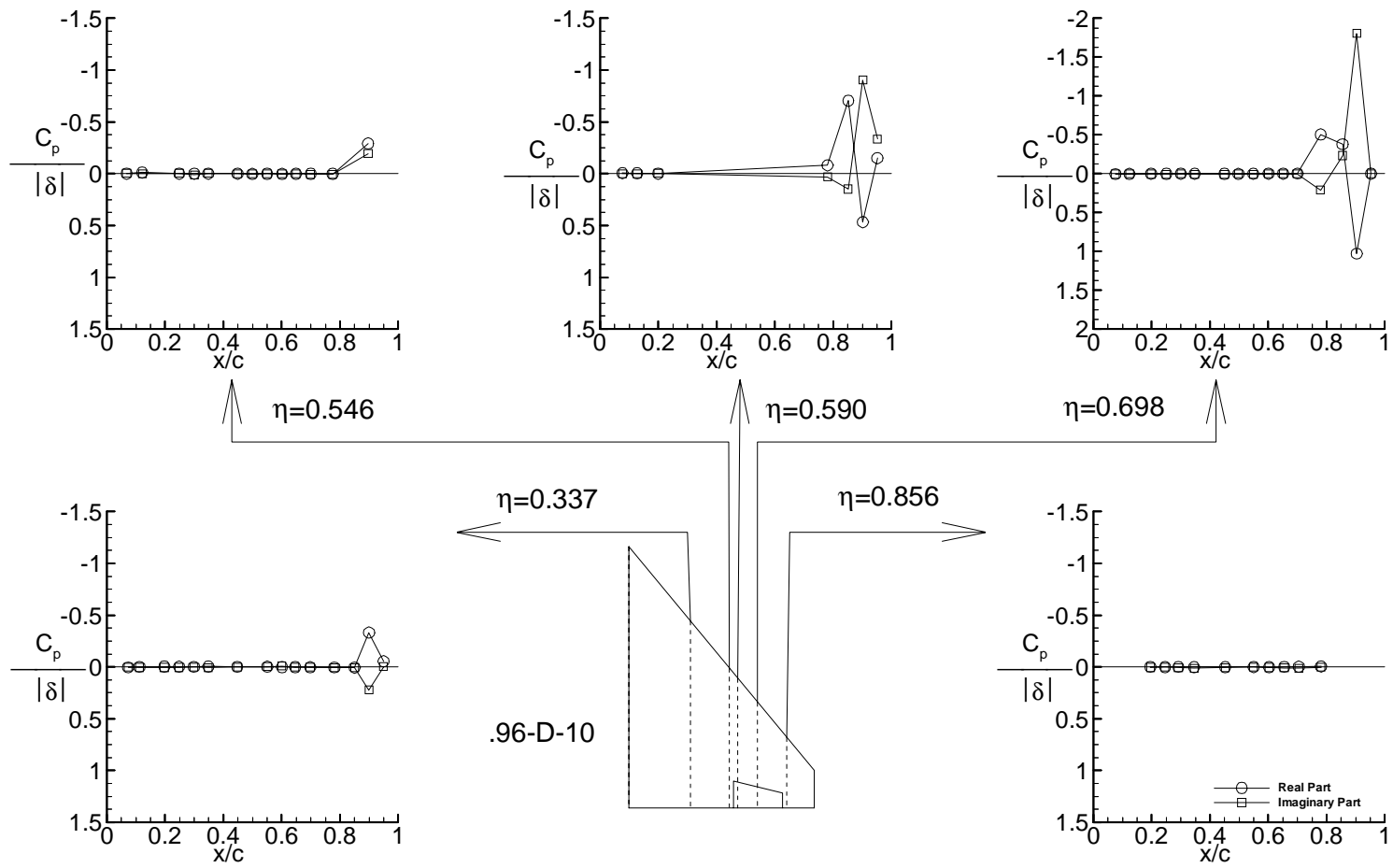
(r-2) Plot of data for test case 9E40 (point .96-D-10) Figure 6. Continued.
