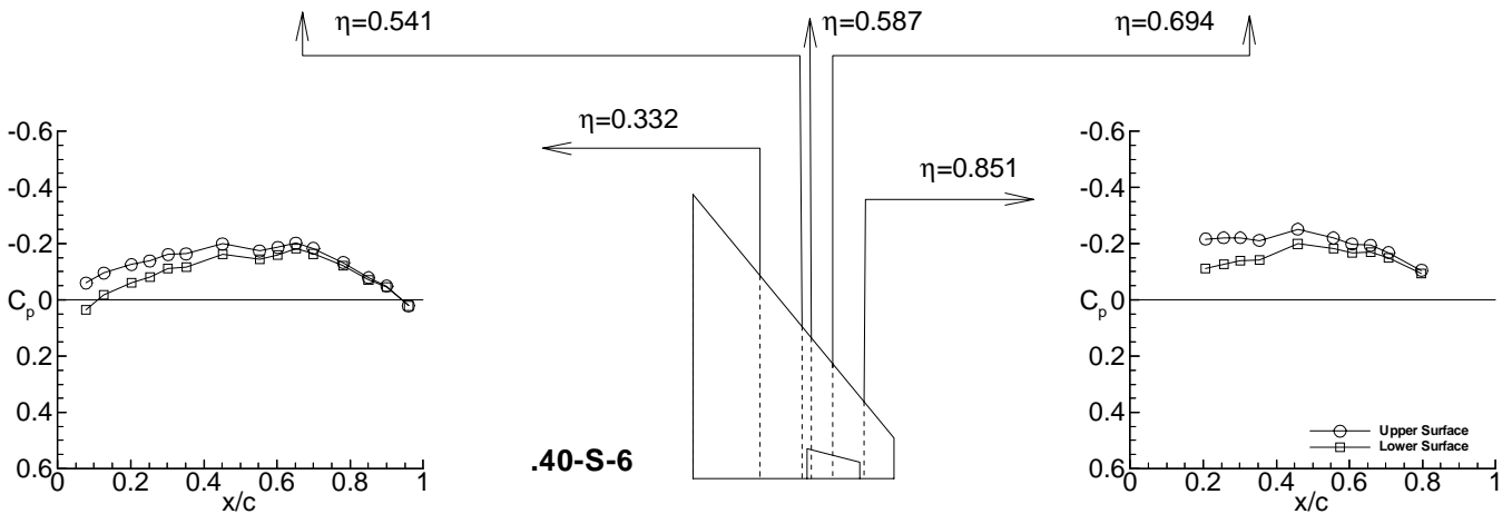
(h) Test case 9E8 (point .40-S-6) Figure 5. Continued.
