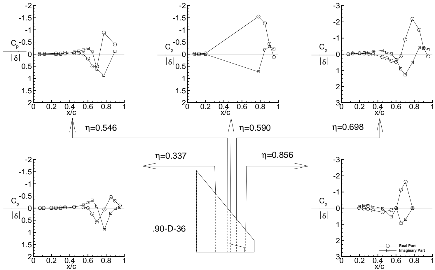
(w-2) Plot of data for test case 9E45 (point.90-D-36) Figure 6. Continued.
