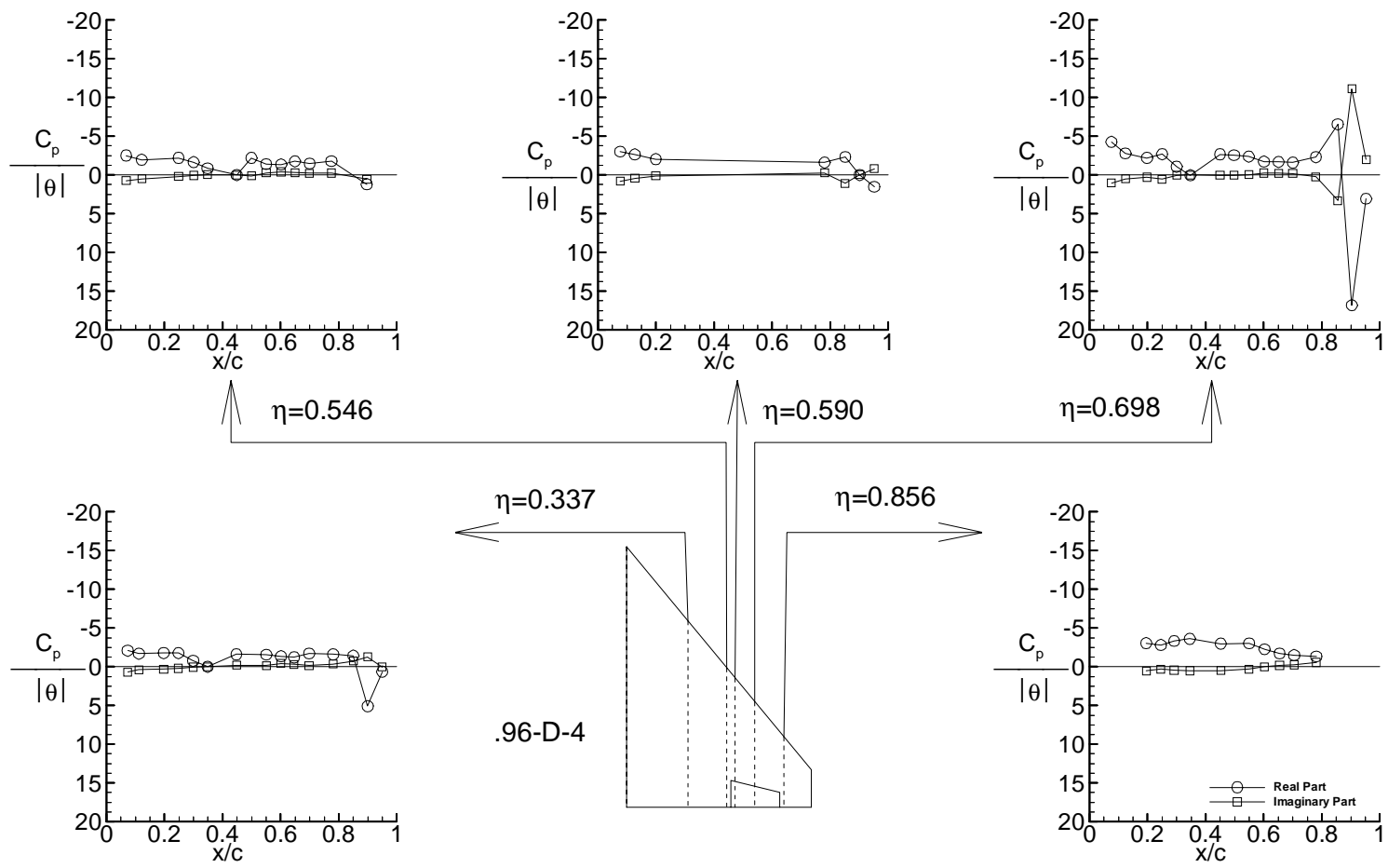
(f-2) Plot of data for test case 9E28 (point.96-D-4) Figure 6. Continued.
