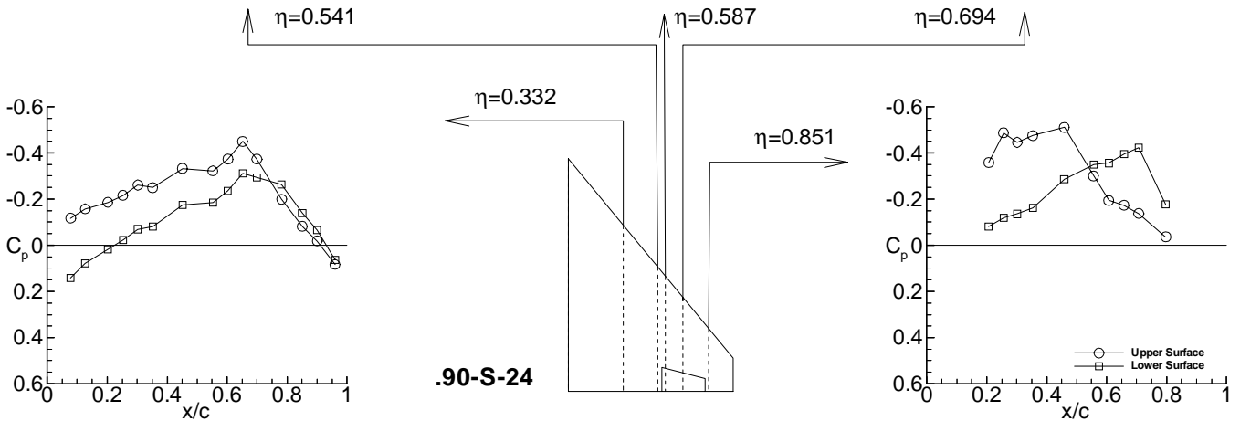
(v) Test case 9E22 (point .90-S-24) Figure 5. Concluded.
