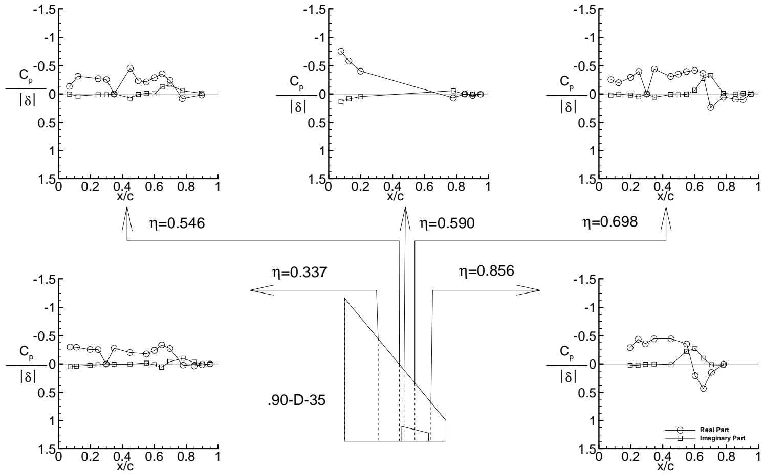
(o-2) Plot of data for test case 9E37 (point .90-D-35) Figure 6. Continued.
