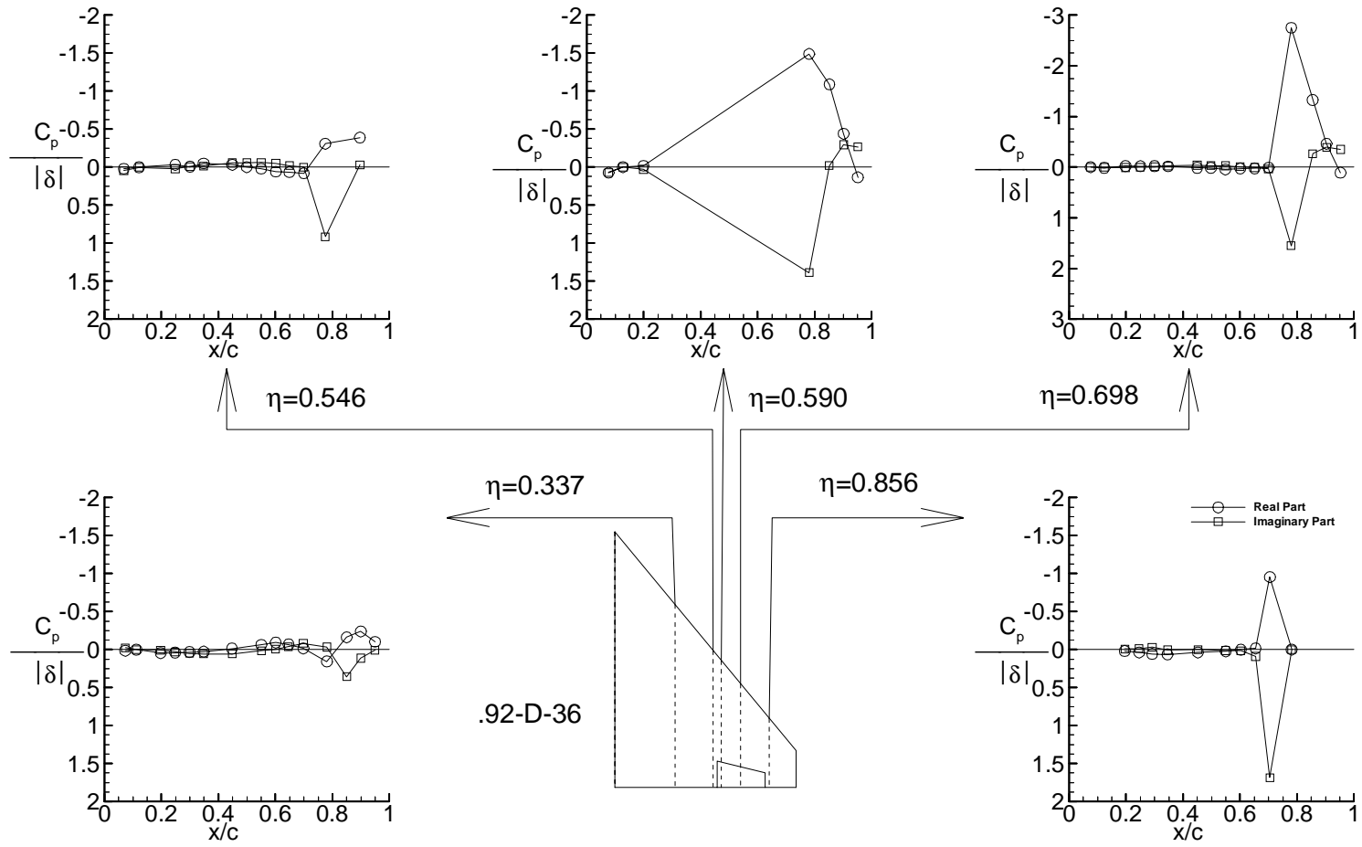
(u-2) Plot of data for test case 9E43 (point.92-D-36) Figure 6. Continued.
