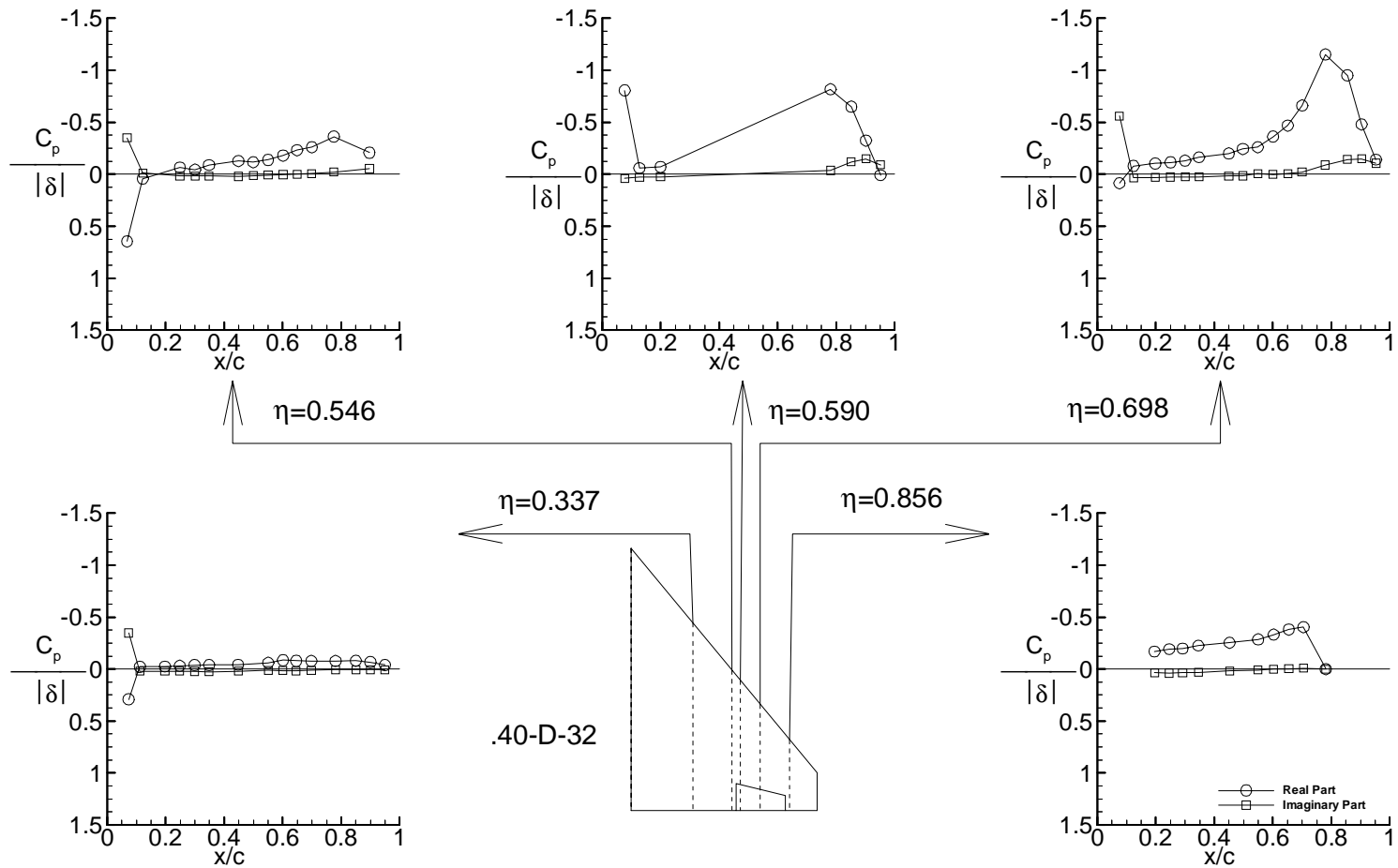
(m-2) Plot of data for test case 9E35 (point.40-D-32) Figure 6. Continued.
