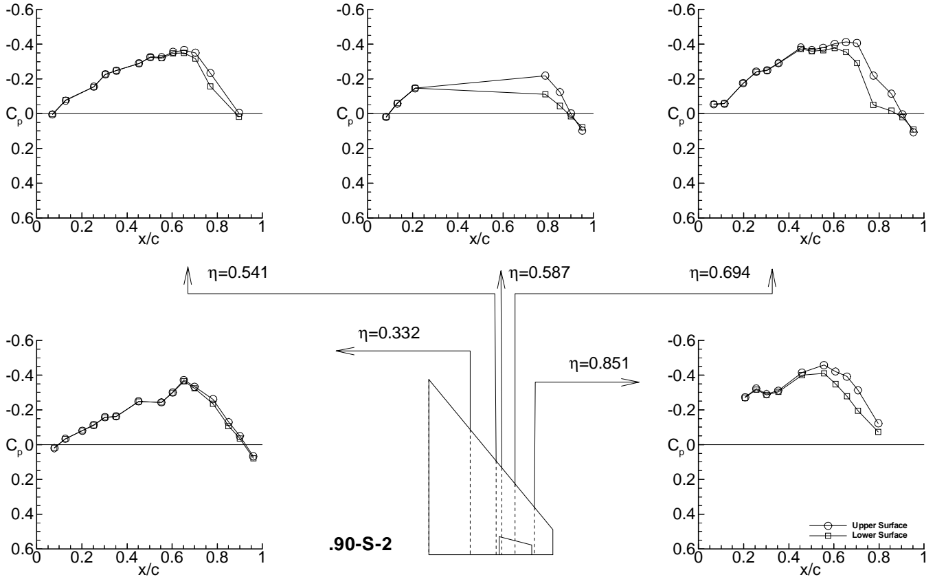
(q) Test case 9E17 (point .90-S-2) Figure 5. Continued.
