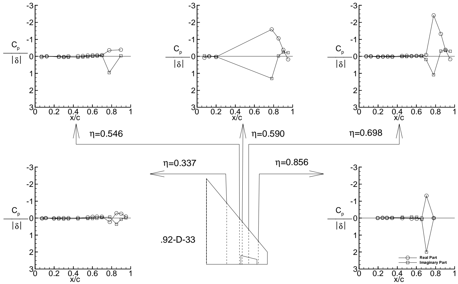
(p-2) Plot of data for test case 9E38 (point.92-D-33) Figure 6. Continued.
