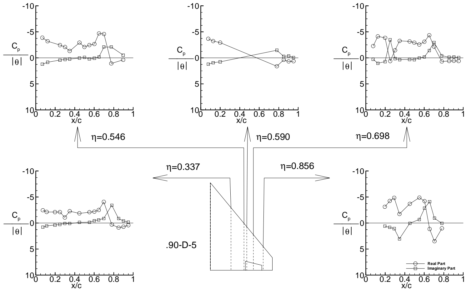
(c-2) Plot of data for test case 9E25 (point.90-D-5) Figure 6. Continued.
