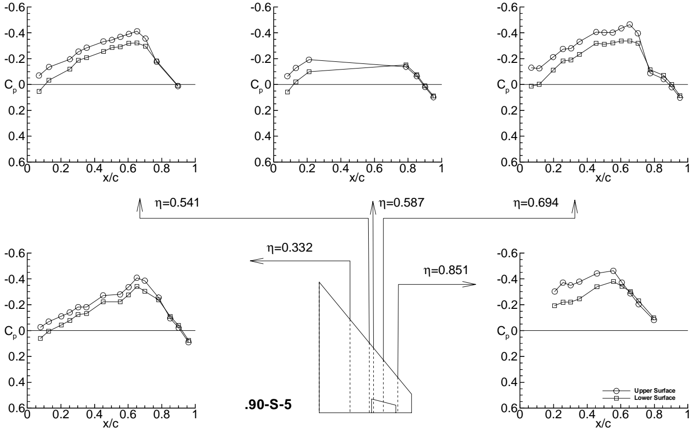
(i) Test case 9E9 (point .90-S-5) Figure 5. Continued.
