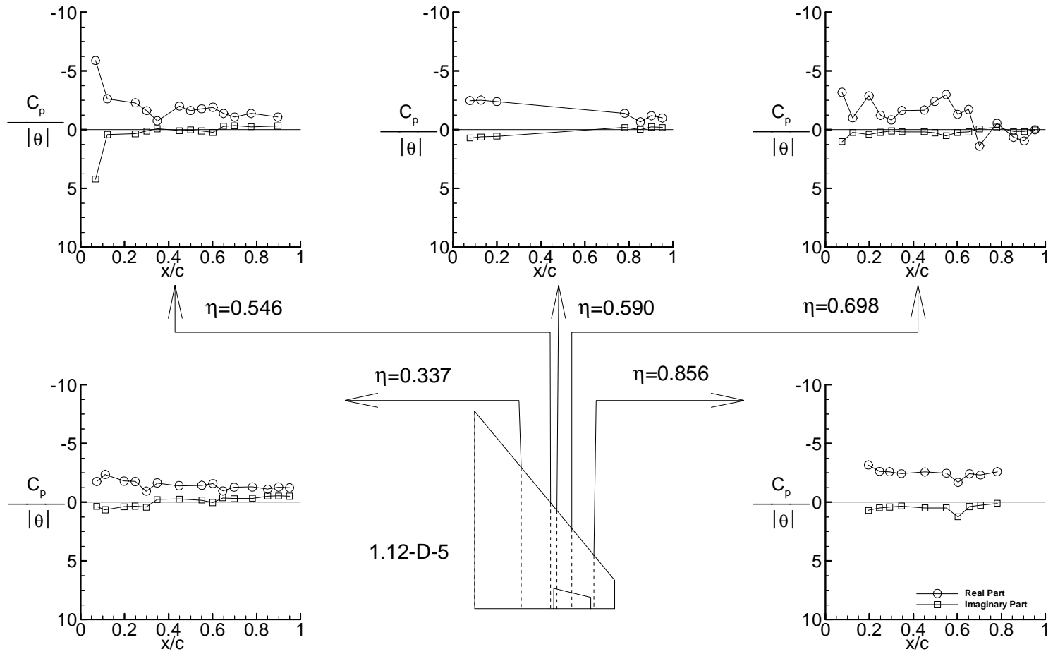
(g-2) Plot of data for test case 9E29 (point 1.12-D-5) Figure 6. Continued.
