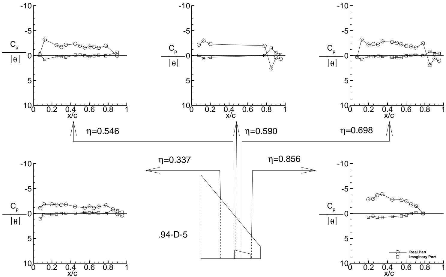
(e-2) Plot of data for test case 9E27 (point.94-D-5) Figure 6. Continued.
