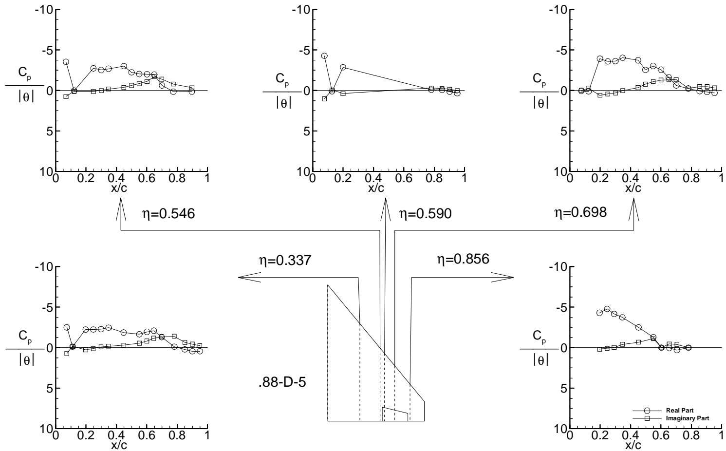
(b-2) Plot of data for test case 9E24 (point .88-D-5) Figure 6. Continued.
