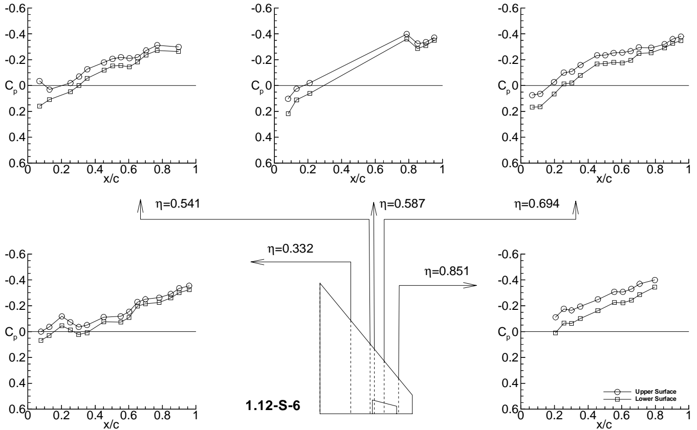
(k) Test case 9E11 (point 1.12-S-6) Figure 5. Continued.
