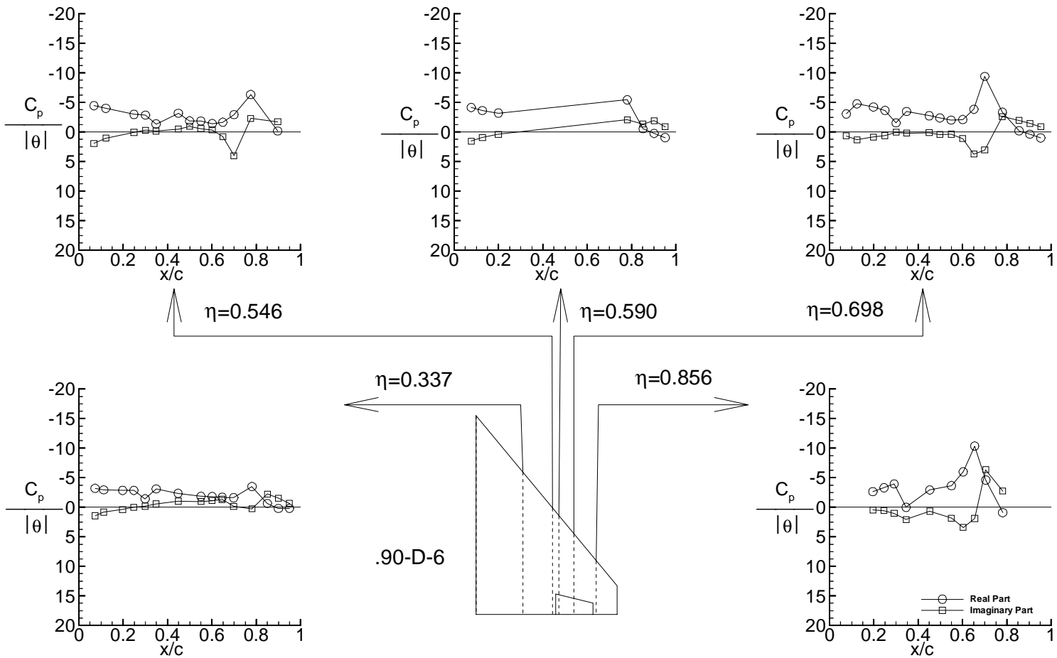
(j-2) Plot of data for test case 9E32 (point 90-D-6) Figure 6. Continued.
